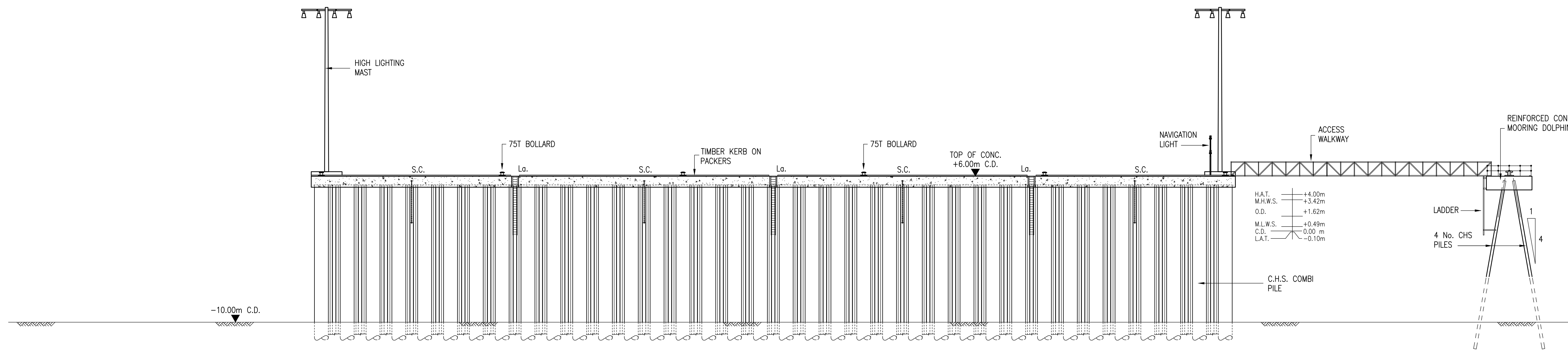
PROPOSED JETTY ELEVATION 1:250
